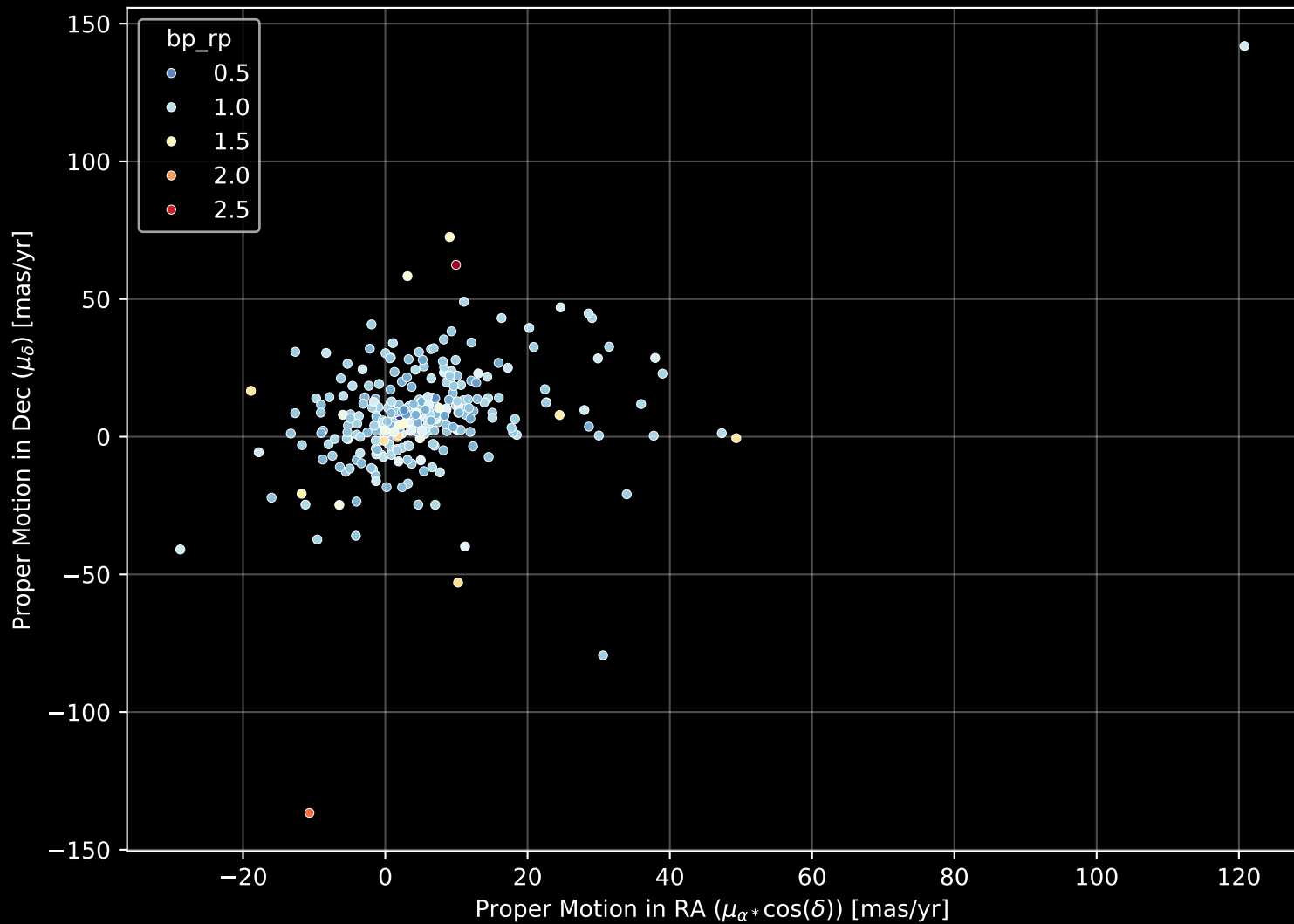
GALAH DR4 Field: [354] Proper Motion Diagram (n= 303)
