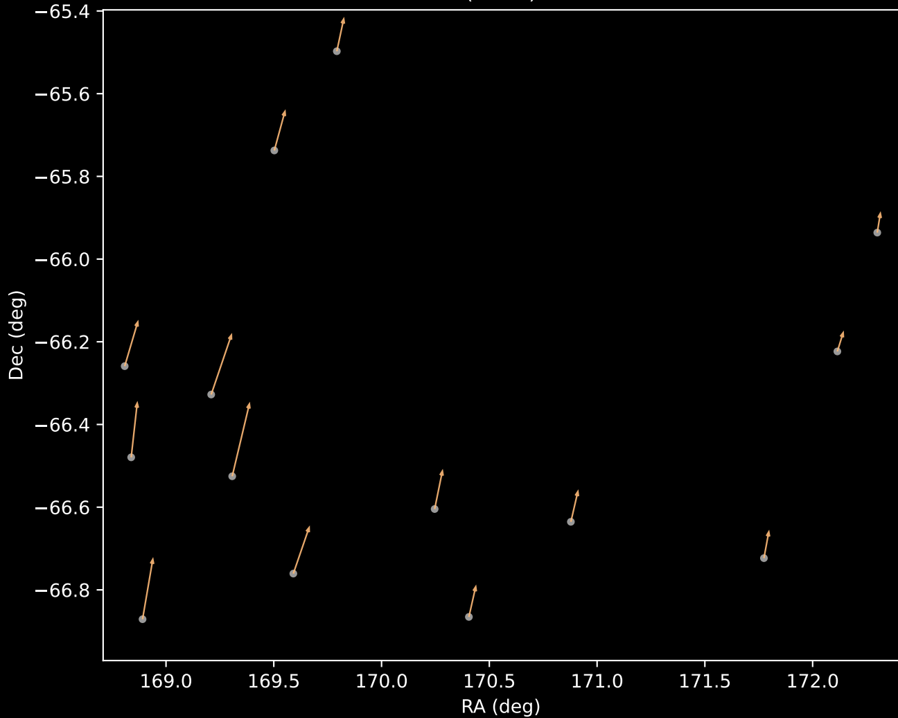
GALAH DR4 Cluster 3 Proper Motion Vectors (n=14)
