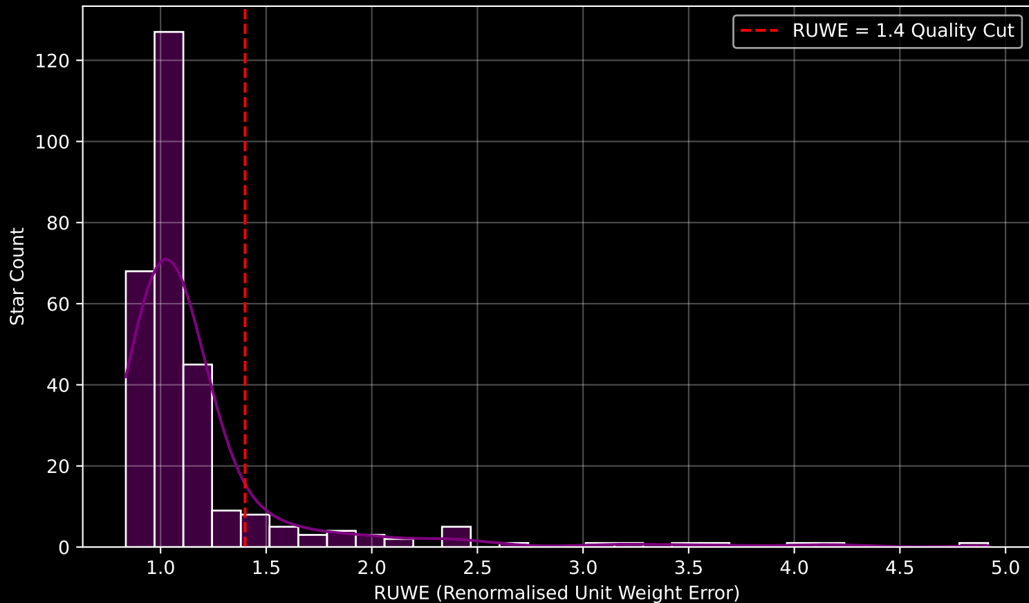
GALAH DR4 Field [354] RUWE Distribution (n= 287)
