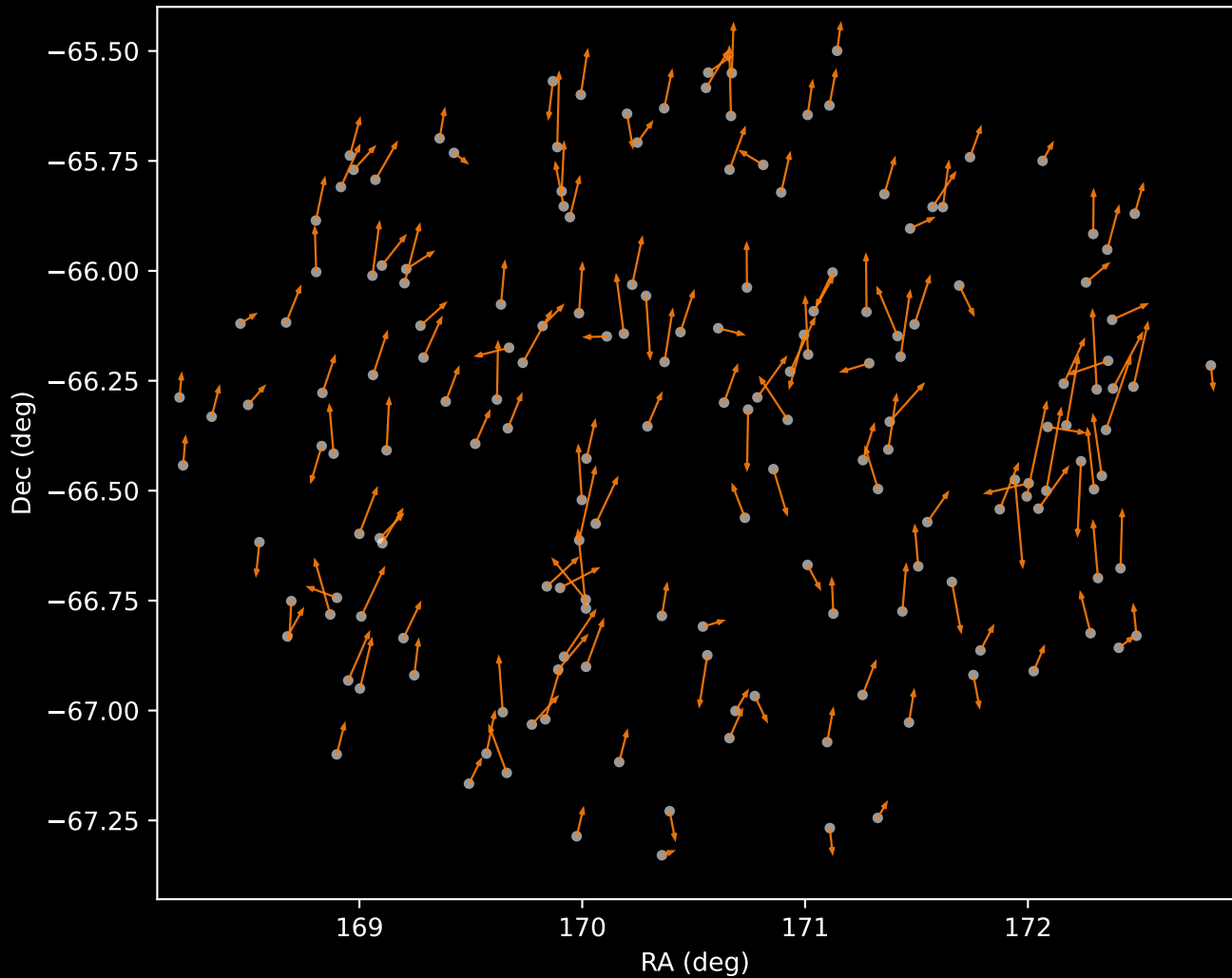
GALAH DR4 Cluster 2 Proper Motion Vectors (n=172)
