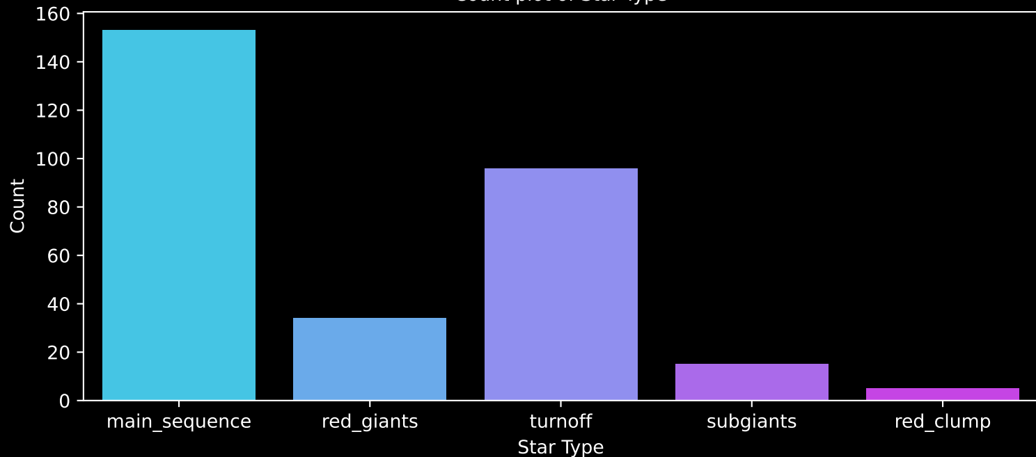
GALAH DR4 Field: [354] Count plot of Star Type
